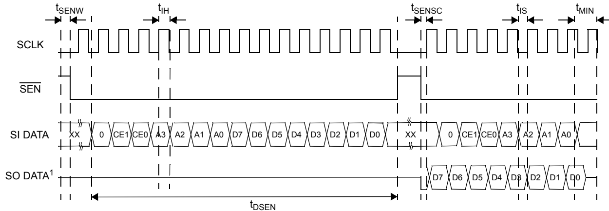
Figure 15: Serial Interface Write Command Timing
